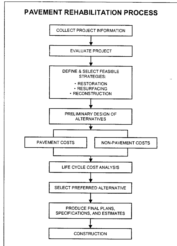
Figure 1. Systematic decision-making process for rehabilitation strategy selection.
