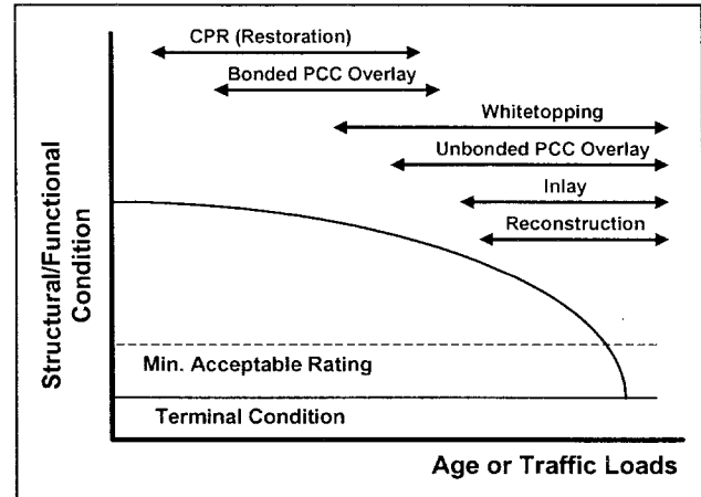
Figure 3. Life-cycle diagram showing how rehabilitation strategies relate to pavement condition.
