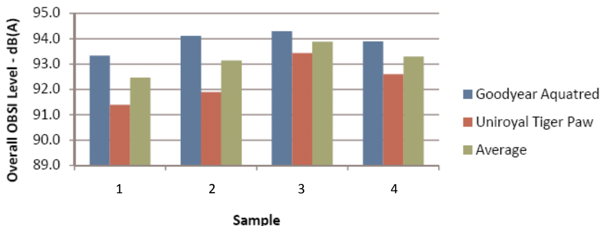
Figure 11 OBSI Results for Samples 1 thru 4 2
