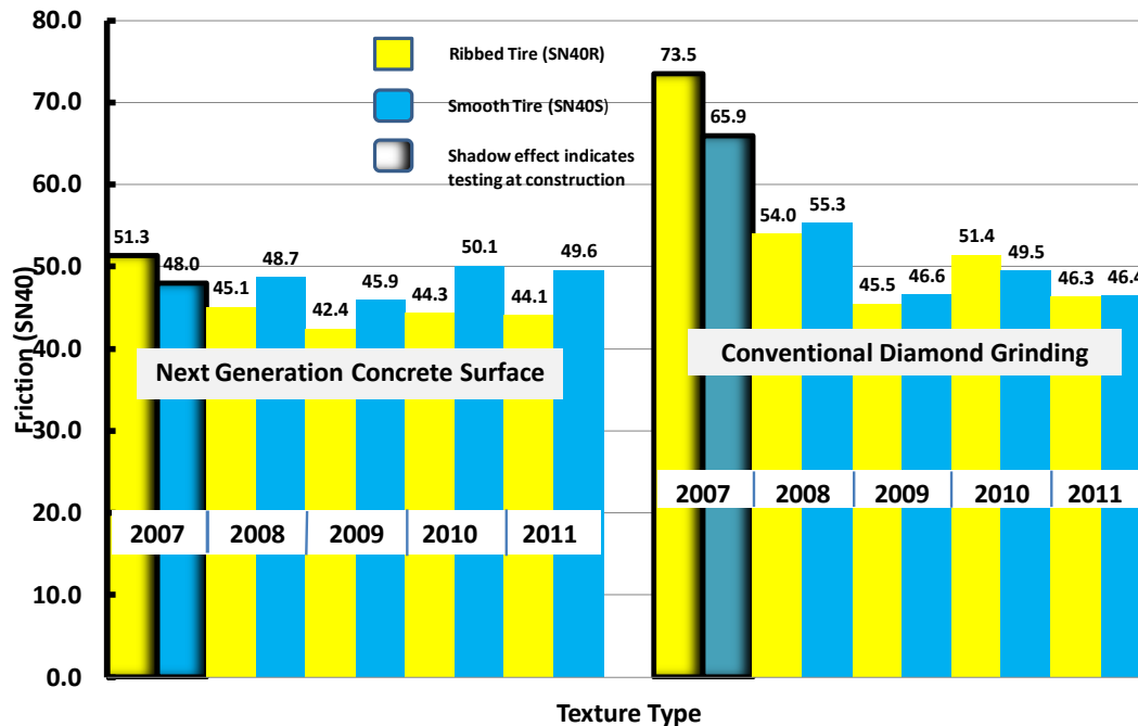
Figure 25 Friction (SN40) as a Function of Surface Texture and Time at MnROAD I-94 WB
