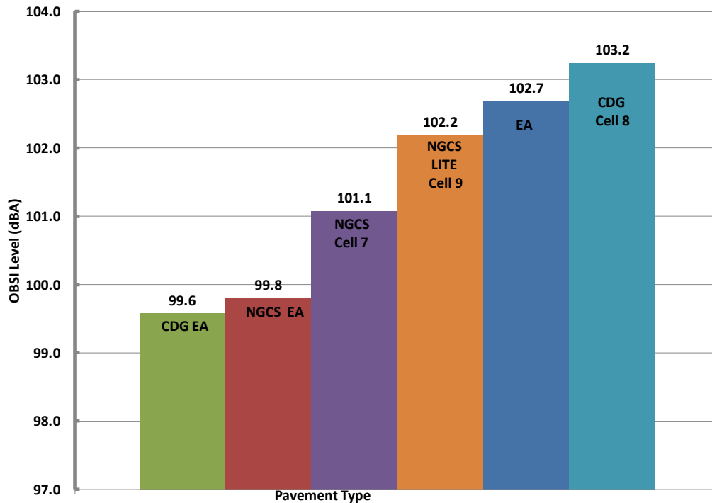
Figure 20 Comparison of Several MnROAD Test Sections to NGCS Test Sections in 2011
