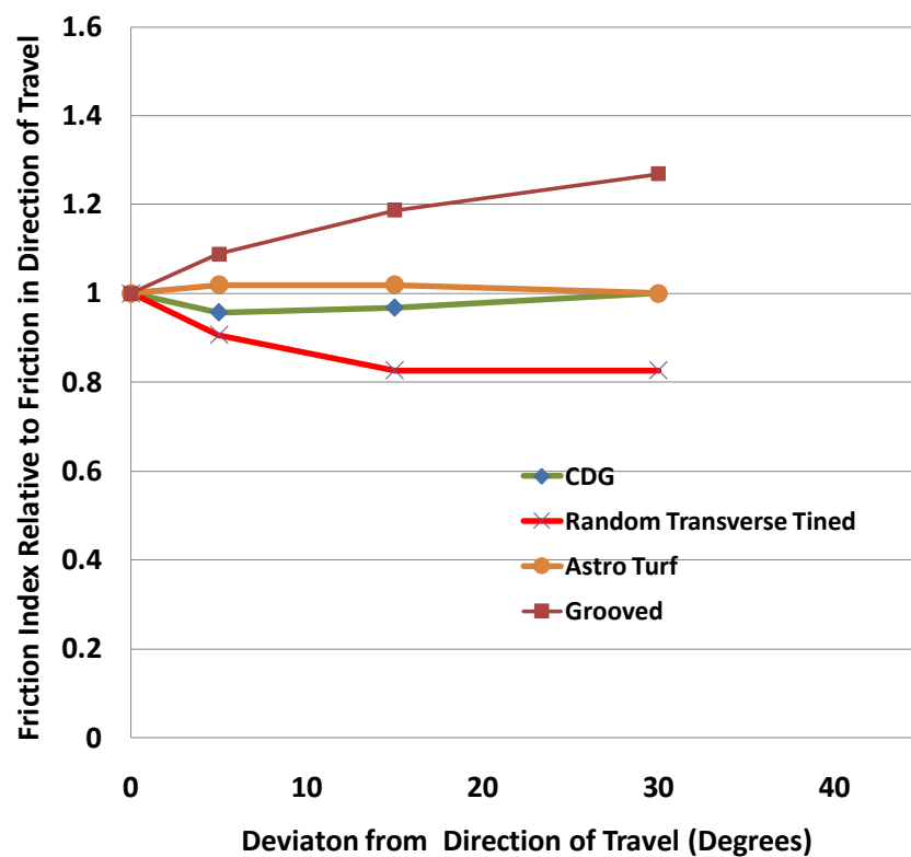
Figure 30 Anisotropic Friction Behavior On Various Concrete Surfaces
