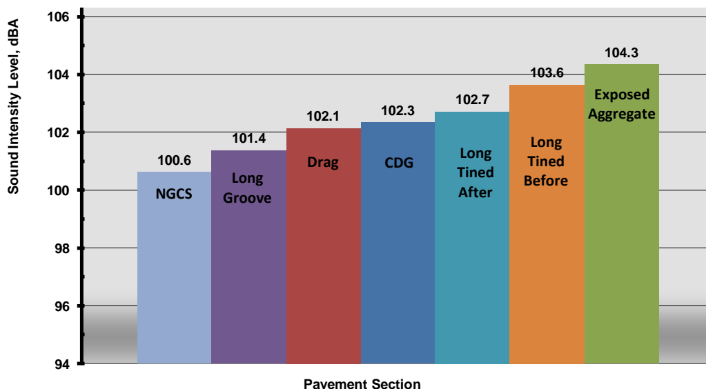
Figure 19 Kansas I-70 EB Surface Texture Test Sections Compared to NGCS in 2011
