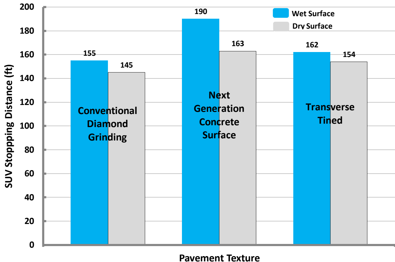
Figure 28 SUV ABS Brake Stopping Distance Testing at Chicago I-355
