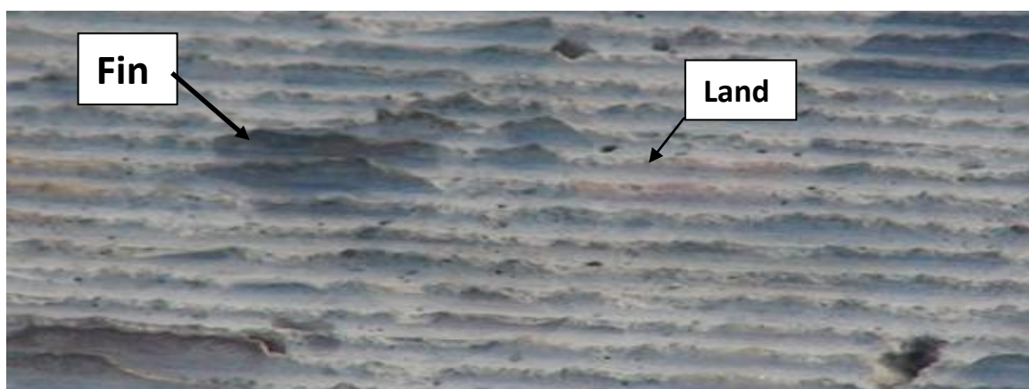
Figure 9- Variability of Fin/Land Profile on CDG Surface on MnROAD I-94
