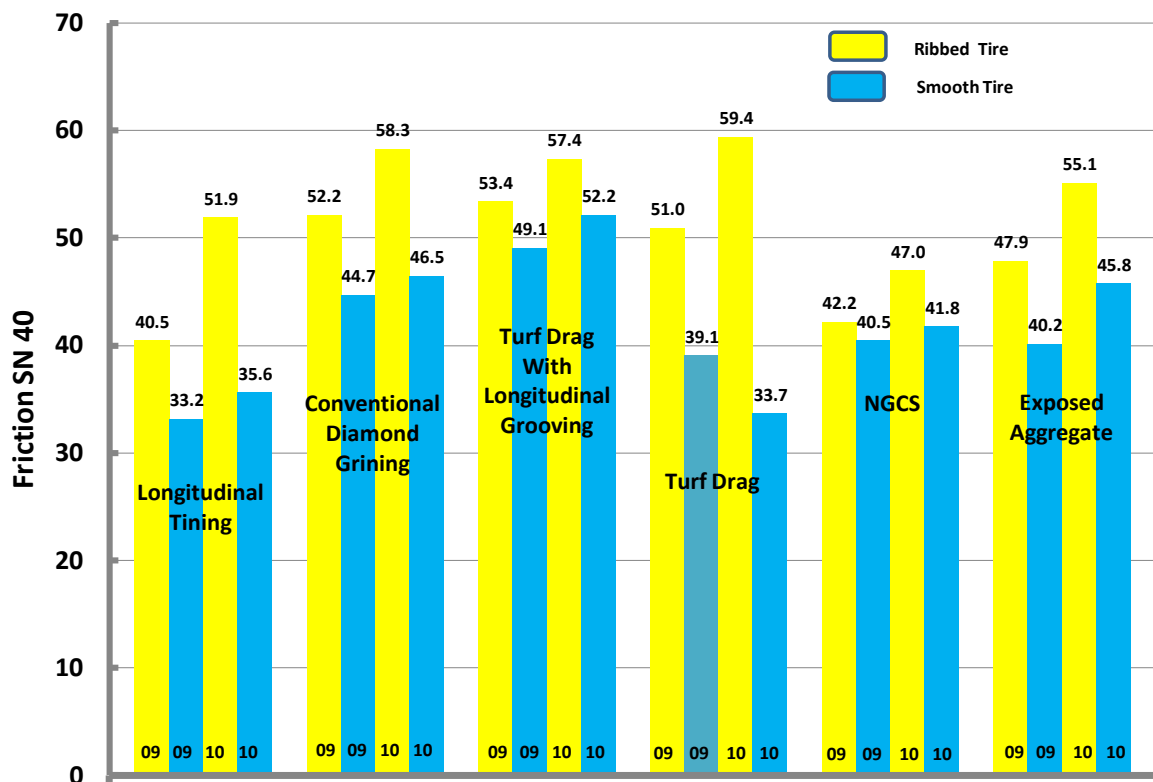
Figure 26 Friction (SN40) as a Function of Surface Texture and Time at KDOT I-70 EB
