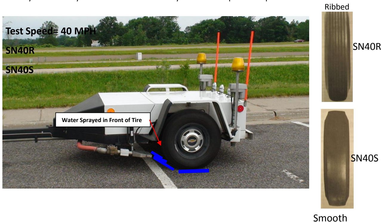
Figure 24 MnDOT ASTM E274 Skid Trailer with ASTM Smooth and Ribbed Tires
