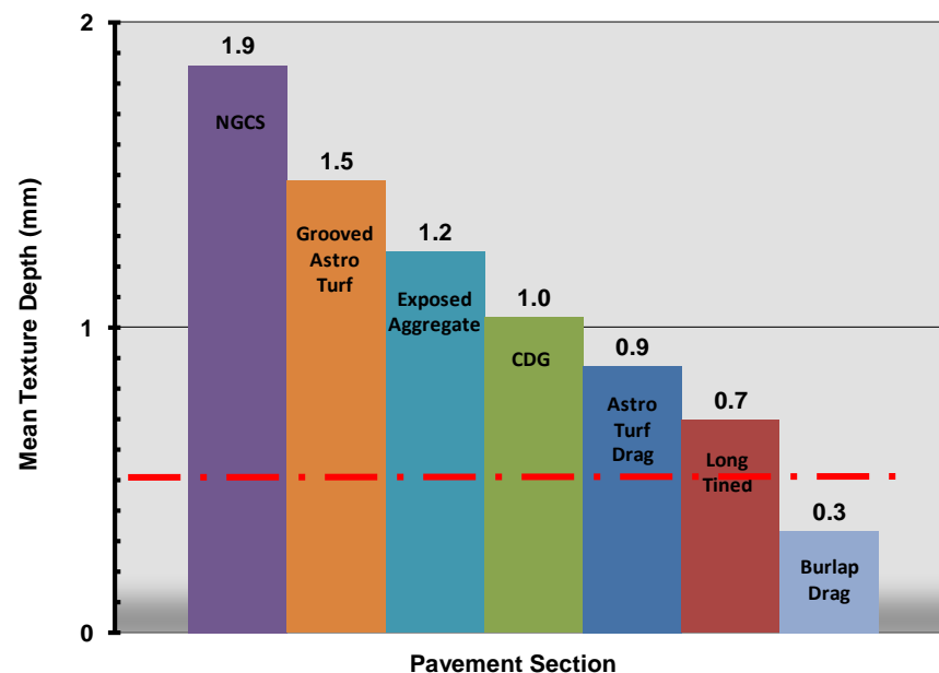
Figure 31 Mean Texture Depths on Kansas I-70 Texture Experiment
